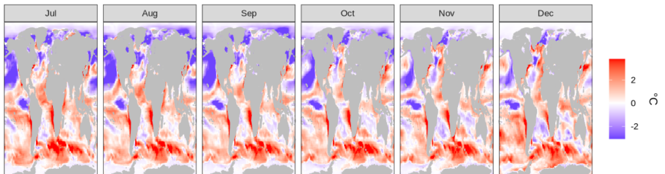
Figure 4: Monthly mean surface sea temperature for the model, observation and the difference between model and observations. For clarity, the maximum values are capped to the 98 th percentiles.
